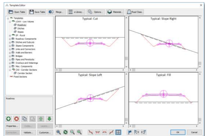
Cross Section Template Editor
